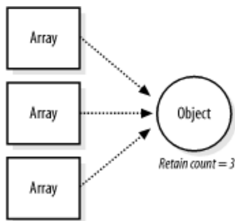
Figure 4-5. Reference counting
