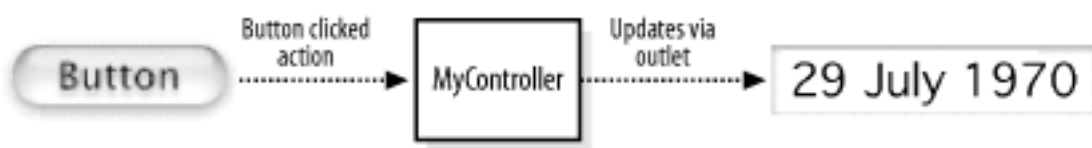
Figure 6-23. Target/action pattern
