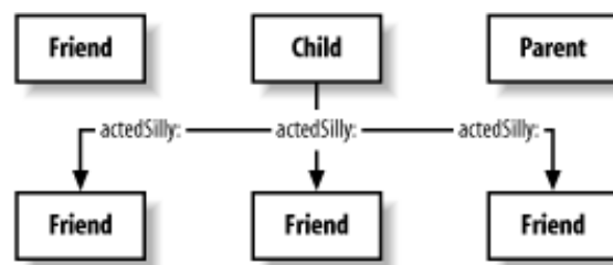
Figure 8-11. Notification
